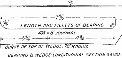
BEARING & WEDGE LONGITUDINAL SECTION GAUGE.
